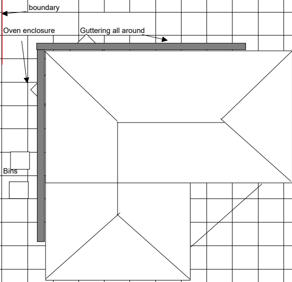
Plan view Roof detail (shown including overhang from wallplate)
