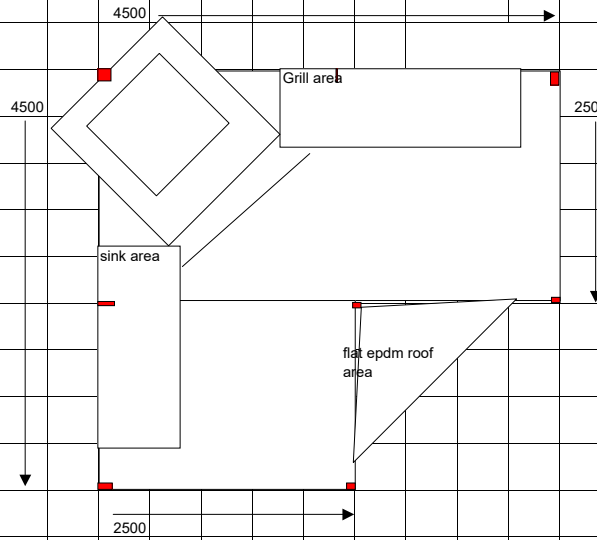
Plan view basic layout (angled corner design)
